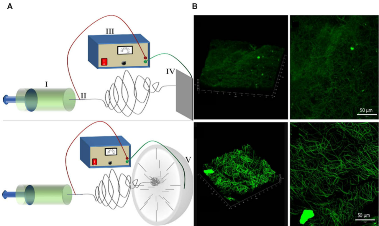
Figure 3. (A) Traditional flat-plate collector, spherical disk and metal array collector. (B) In three-dimensional rendering and two-dimensional projection, a cotton ball-like ePCL scaffold has a loosely packed network structure [116]. Copyright 2011 Elsevier.
