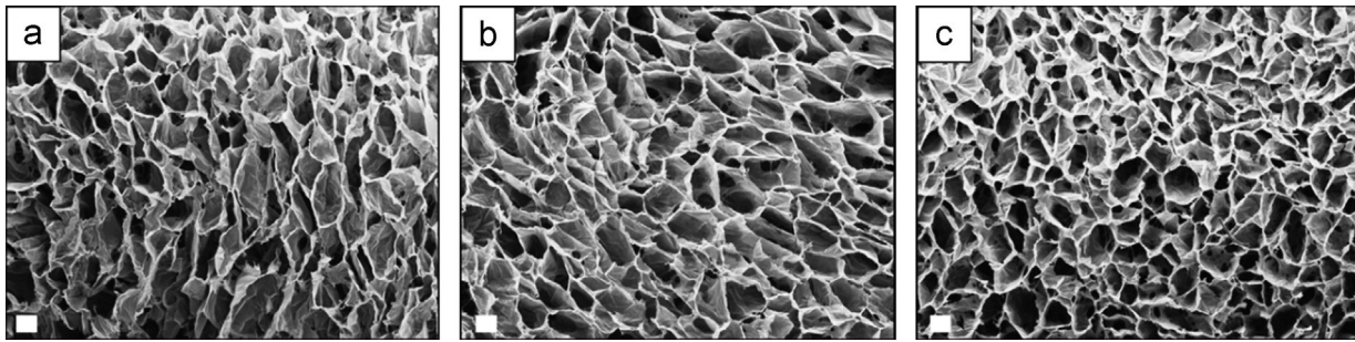
Fig. 2 – Freeze-dried collagen scaffolds, vertical cross-section, (a) 0.5% w/V, (b) 1% w/V in silicone molds, and (c) 1% w/V in stainless steel molds. The scale bar is 100 \mu\text{m} .
