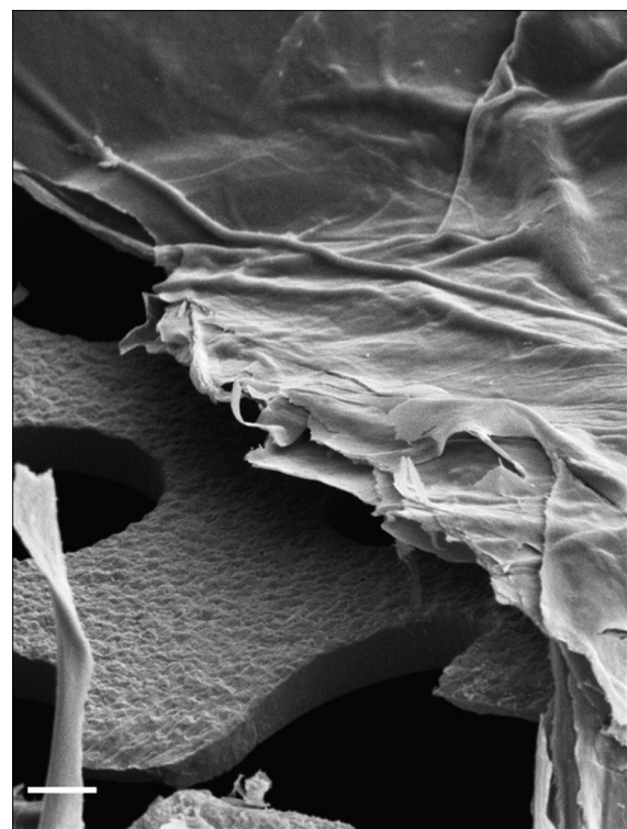
Fig. 5 – 1% w/V in silicone molds membrane deposited on a copper grid. A stack of single pore walls can be seen lying parallel to the substrate. Scale bar is 10 \mu\text{m} .
