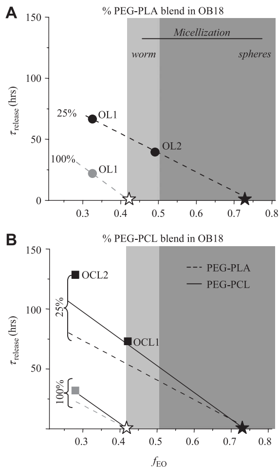
Fig. 7. Summary of encapsulant release kinetics from copolymer vesicles as dictated by both chain chemistry and PEG volume fraction ( f_{\text{EO}} ). (A) OL copolymers of several thousand g/mol can integrate at 25 mol% into stable vesicles of inert OB18 as long as f_{\text{EO}} \leq 0.73 (gray-filled star). For pure vesicles of such degradable copolymers (i.e. 100%), release is much faster and requires f_{\text{EO}} \leq 0.42 (open star). (B) OCL copolymer of similar M.W. to OL1 and OL2 degrades more slowly when accounted for the f_{\text{EO}} effects. This delay due to polyester chain chemistry reflects retarded PCL degradation kinetics. A characteristic release line through the result for the 25% OCL blend intersects the 25% OL line at f_{\text{EO}} = 0.73 , where f_{\text{EO}} dominates any major difference in degradation chemistry. Likewise, release from pure OCL vesicles can be predicted by postulating slower proportionate degradation but at a common microphase stability limit of f_{\text{EO}} = 0.42 . Comparing the two OCL1 lines to OCL2 data points reveals the M.W. effect or lack thereof since OCL2 is about four-fold bigger than OCL1 and the two OL block copolymers.
