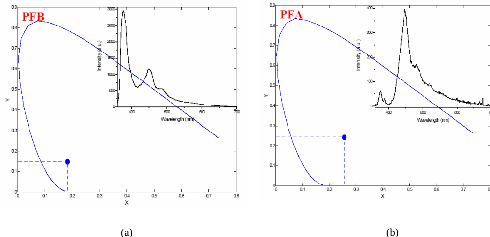
Fig. 5. Tristimulus color coordinates of (a) PFB-hybridized LED (Control) with CRI of 53 and (b) PFA-hybridized LED (Sample 3) with CRI of 91 respectively, along with their optical emission spectra in the inset when their respective integrating LEDs are electrically driven.
