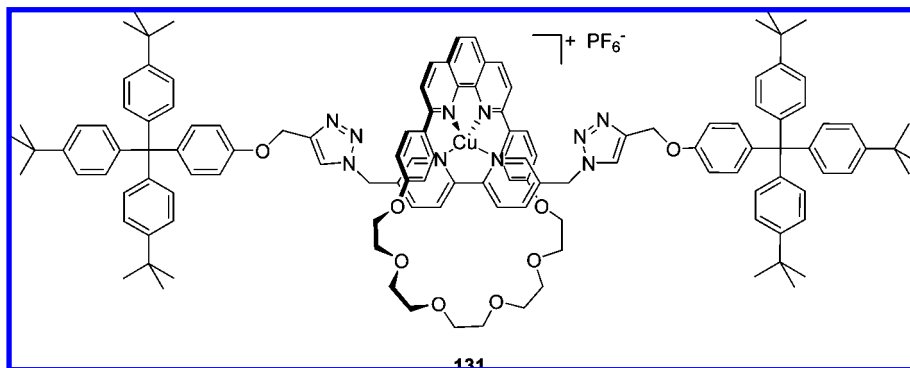
Figure 24. During stopper conjugation through CuAAC the bis-azide was held in place by bipyridine coordination, giving a high yield of roxatane 131 .
