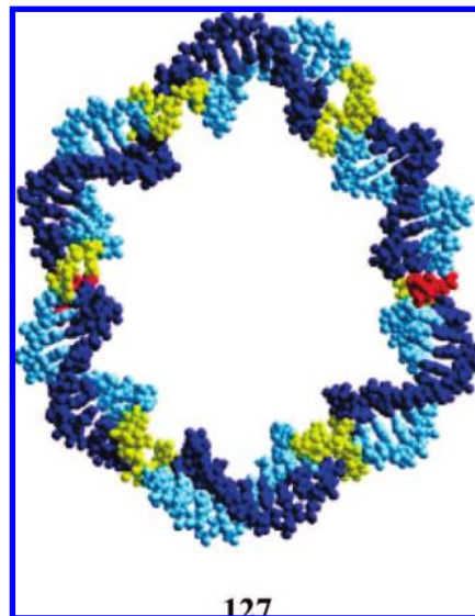
Figure 21. Formation of a double-stranded pseudo-hexagon from a single stranded cyclic template generated by triazole coupling (red) and linear precursor to entwine and cyclize the second strand with a triazole coupling (red). The single-strands are entwined six times. Unpaired TpT/TpT hinge segments are shown in yellow and double-stranded regions in light and dark blue. Reprinted with permission from ref 269. Copyright 2007 American Chemical Society.
