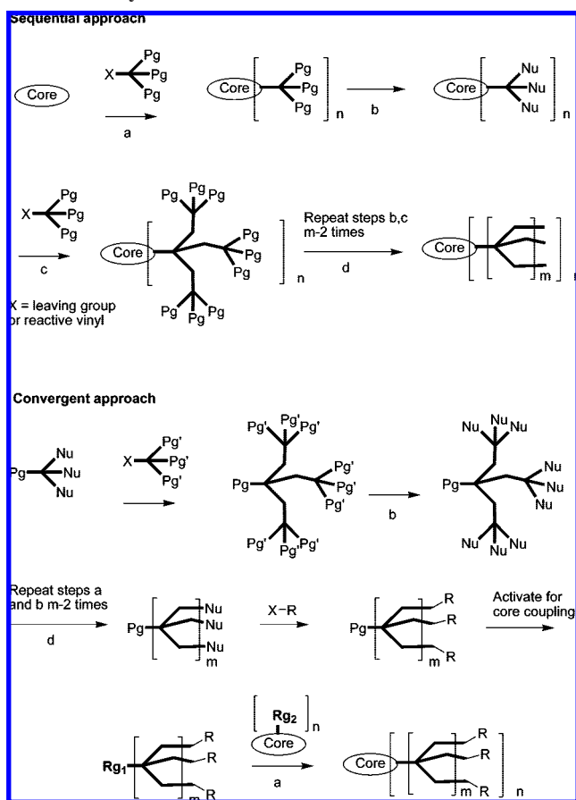
Figure 27. Putative core architectures for CuAAC. Many of these have been used in dendrimers synthesis.
