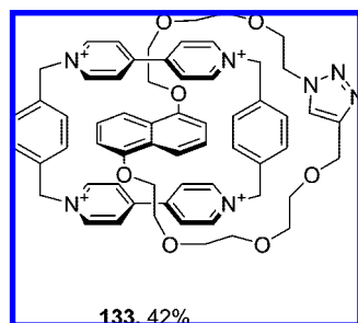
Figure 26. Catananes may be synthesized by CuAAC from precursors similar to those for compound 132 .
