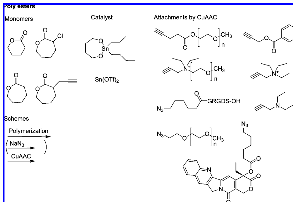
Figure 46. Polyesters can be formed by ring opening polymerization reactions starting from \alpha -substituted caprolactones. The chloro-substituted polymer can be converted to the azide containing polymer in high yield, and the azide can be used for CuAAC functionalization.
