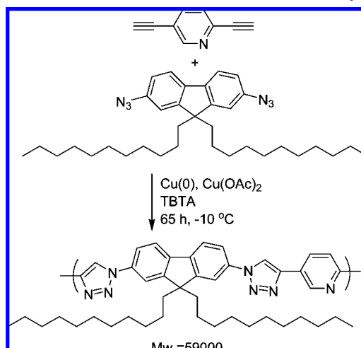
Scheme 28. Conjugated Polymers Were Formed through CuAAC of Aromatic Bisazides with Aromatic Bisalkynes a
