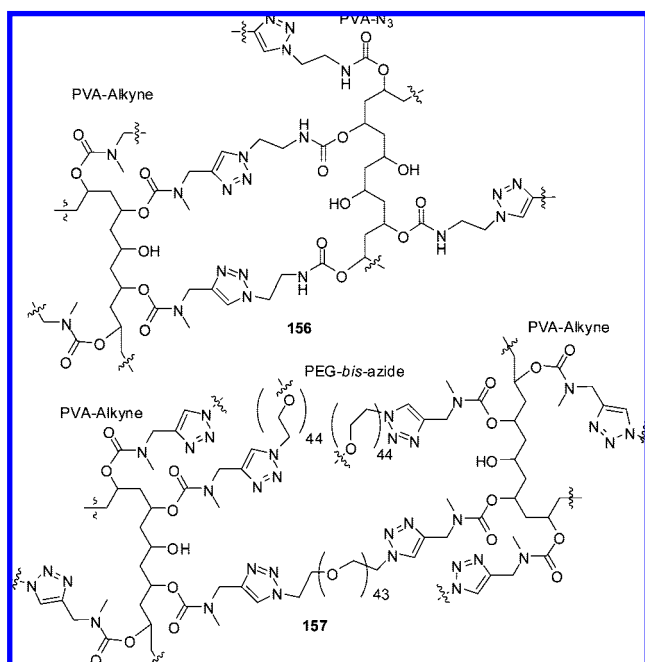
Figure 52. Cross-linked polymers were synthesized from linear poly(vinyl alcohols) and PEG polymers. The property of the final polymer may be tailored by substitution density of functional groups and polymer length.
