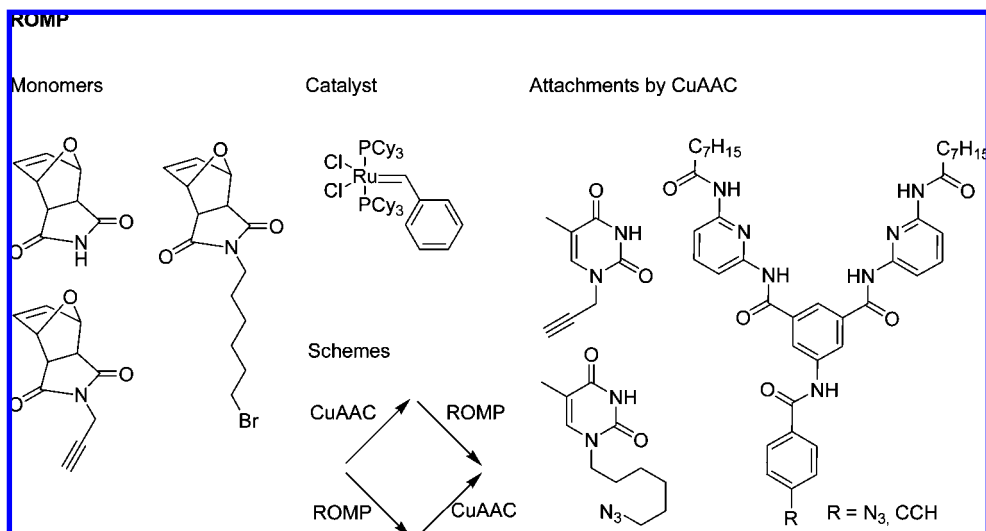
Figure 44. ROMP is an orthogonal polymerization technique that is very useful for preparation of polymers carrying a variety of functional groups including alkynes and alkyl halides easily converted to azide for CuAAC.
