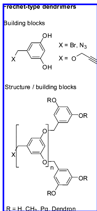
Figure 29. The Fréchet-type of dendrimer structure.
