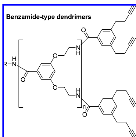
Figure 32. The benzamide-type of dendrimer structure.
