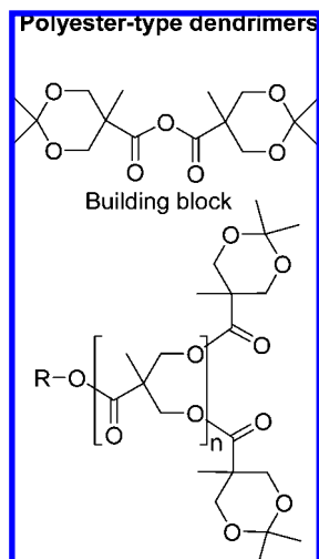
Figure 31. The polyester-type of dendrimer structure synthesized from the acetone of 2,2-di(hydroxymethyl)propanoic ester.
