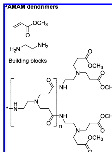
Figure 30. The PAMAM dendrimer structure.
