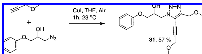
Scheme 4. Reaction of Electrophiles with Copper-Triazole Adduct 5
