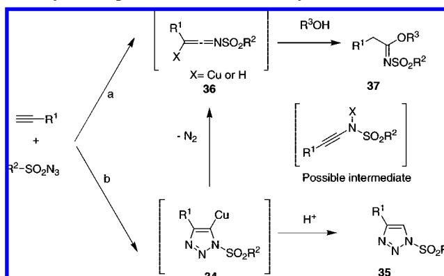
Scheme 5. In CuAAC with Sulfonyl Azides, the Cu-Triazole 34 May Decompose To Form the Sulfonylketimine 36
