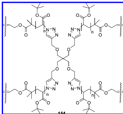
Figure 50. A cross-linked polymer that forms soluble star polymers by ozonolysis was synthesized by reacting bis-azide polymers formed from a divalent initiator with a tetravalent azide cross-linking agent using CuAAC.
