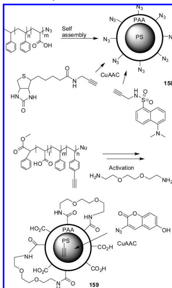
Scheme 31. Core–Shell Nanoparticles Produced by Self-assembly of Amphiphilic Block Copolymers May, if They Contain Azide or Alkyne in the Core or Shell, Be Modified Selectively at These Sites
