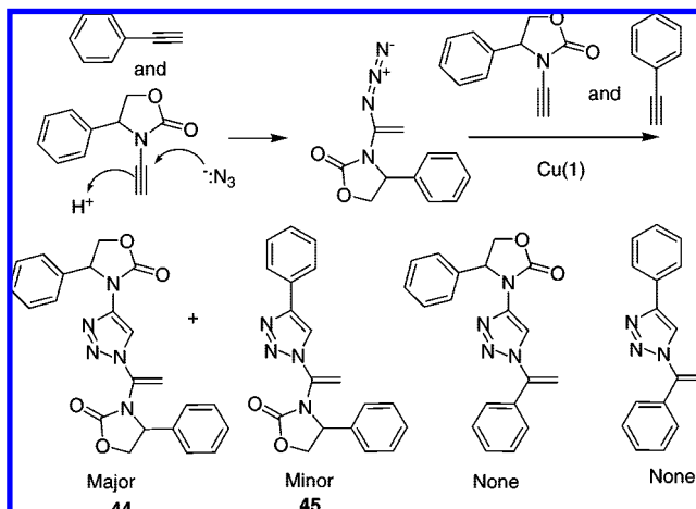
Scheme 7. The Competing Hydroazidation Reaction, Which Is Observed as a Side Reaction in Reactions of Ynamides with Azides (the Normal Azide/Alkyne Reaction Is Not Shown) a
