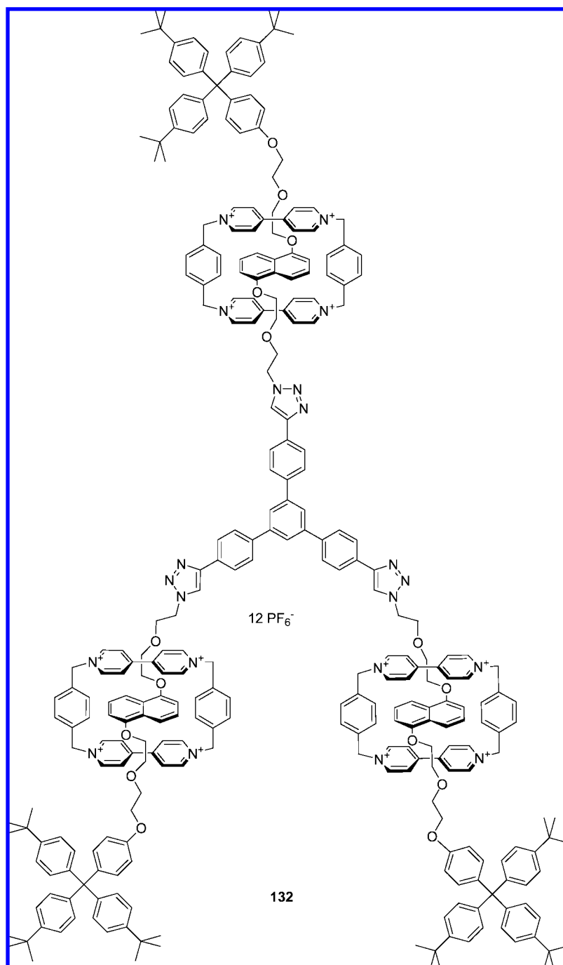
Figure 25. Tripodal rotaxane obtained in 62% yield through CuAAC.
