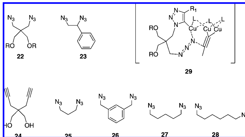
Figure 6. Bis-azides 22 and 23 gave considerable rate enhancement for formation of the second triazole. Compounds 24 – 28 do not have this ability to any significant extent. The rate enhancement could occur via intramolecular coordination of the second azide to the Cu(1) cluster, leaving the first formed triazole.
