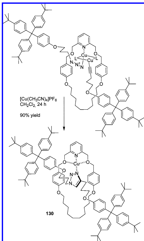
Scheme 23. The Synthesis of Rotaxanes Has Been Facilitated Greatly through CuAAC That Helps Coordinate the Two Reaction Partners in the Arch of the Macrocycle by Auxiliary Coordination of the Catalytic Cu(I)
