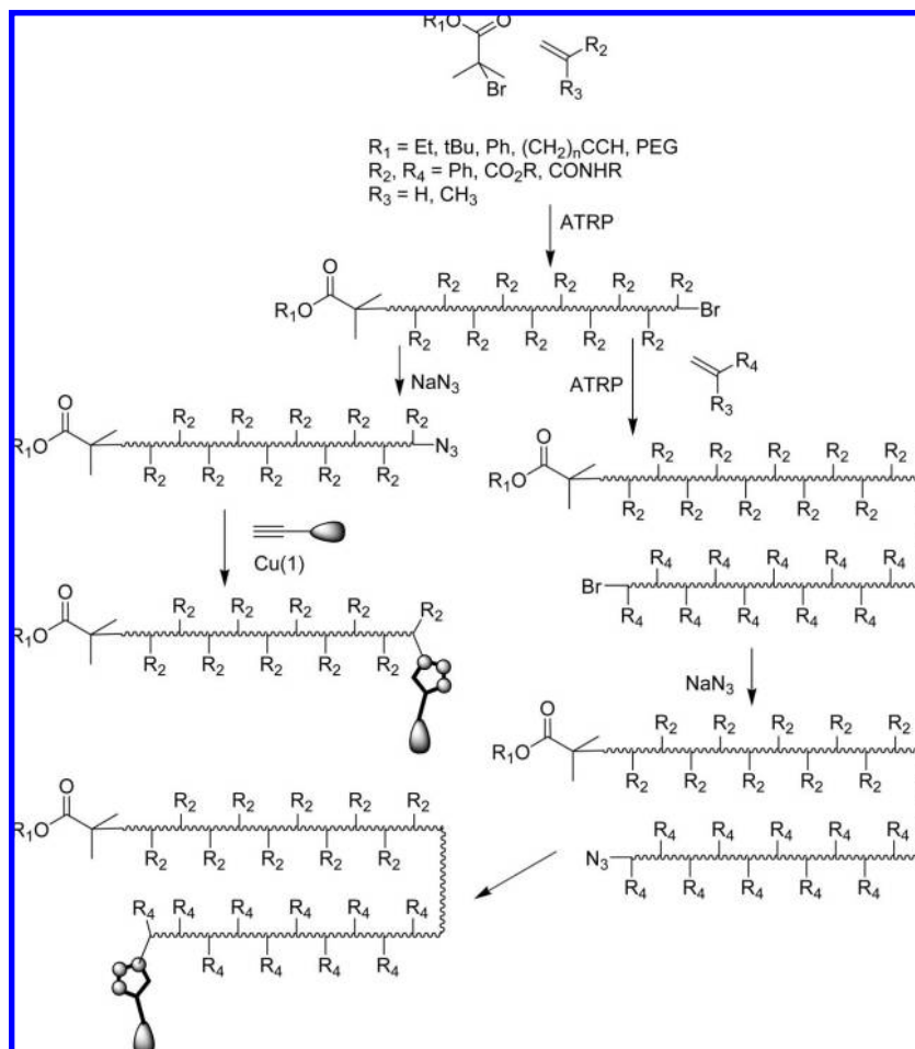
Scheme 26. Controlled Living Polymerizations Allowing Both Block Copolymers and Specific Terminal Modification of the Polymer by CuAAC
