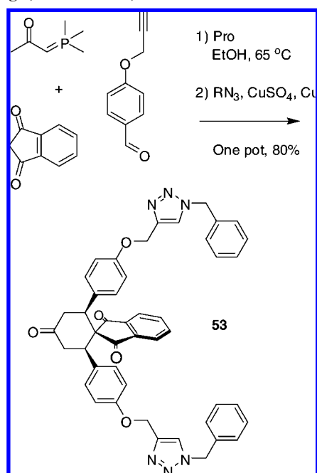
Scheme 13. One-Pot Reaction Involving Wittig, Knoevenagel, Diels–Alder, and CuAAC Reactions
