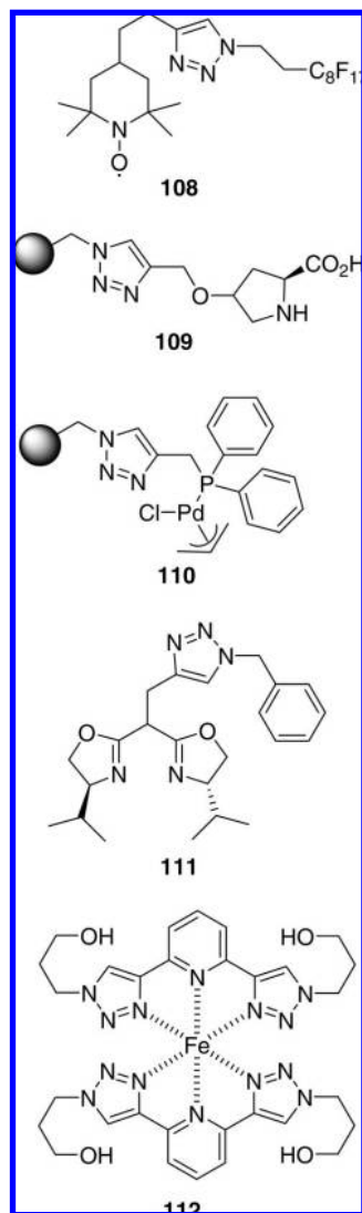
Figure 17. Catalysts and metal ligands derived through CuAAC.
