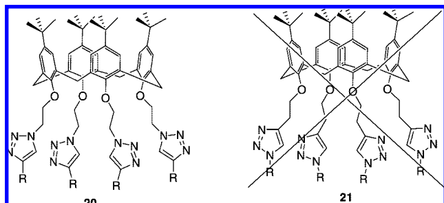
Figure 5. For calixarenes decorated with azidoethyl ethers the Cu(I) catalyzed reaction with alkynes forms four triazoles simultaneously in a total yield of 80% while the same calixarene decorated with alkynes failed to give the expected product.
