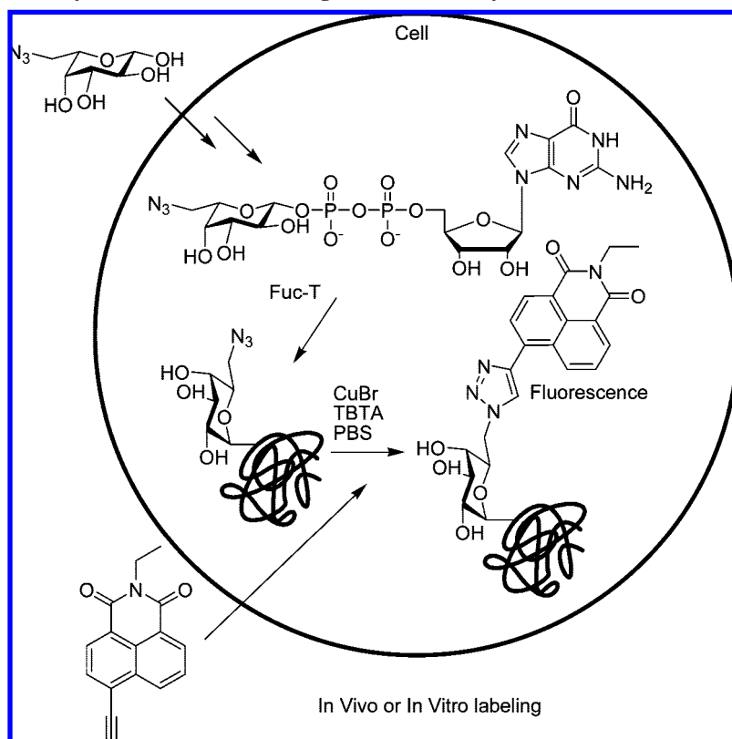
Scheme 34. In Vivo CuAAC May Facilitate the Monitoring of Fuc-T Activity in the Cell a
