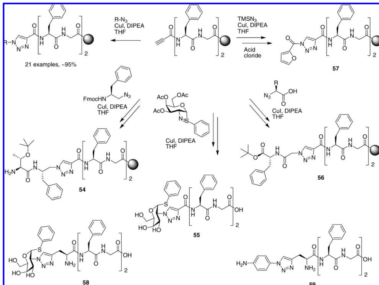
Scheme 14. The Versatility of the CuAAC Was Demonstrated through Synthesis of a Large Variety of Differently Linked Peptidic Triazoles, e.g. 54–59 on Solid Support in Essentially Quantitative Yield
