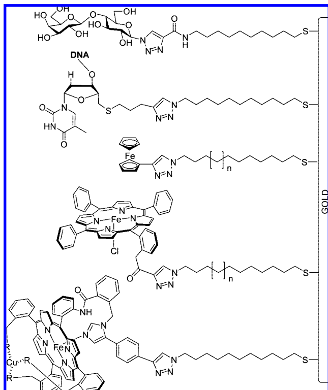
Figure 55. Gold surfaces have been modified with complex molecular entities for voltametric measurements and plasmon resonance. A special application is that of controlling the derivatization locally through reduction of Cu(2) to Cu(1) over a microelectrode kept at -300 mV with reference to the solution.
