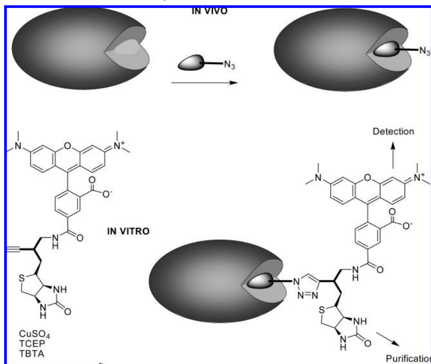
Scheme 33. Activity Based Protein Profiling Employs Specific Covalent in Vivo Attachment of a Small Molecule Containing an Azide or Alkyne to the Active Site of a Protein Family or Class a
