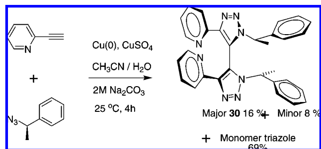
Scheme 2. Oxidative Coupling To Yield up to ~90% Bis-triazoles Can Be Promoted by the Presence of Inorganic Base and Air a
