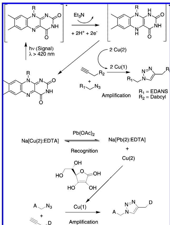
Scheme 18. CuAAC Can Be Used as a Coupled Amplification Reaction To Detect a Signal or a Molecular Recognition Resulting in Formation of Cu(1)
