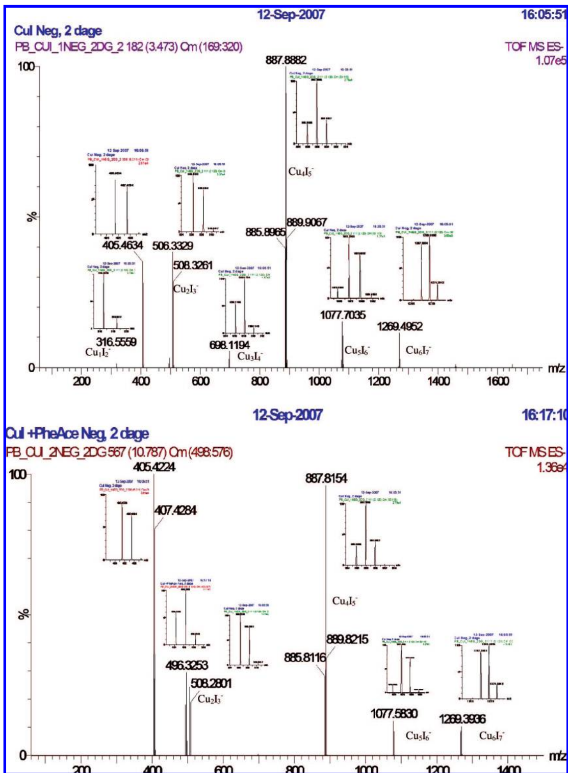
Figure 2. ESI-MS (Micromass QTOF-Ultima, negative mode, collision energy 10) of a 100 \mu M solution of CuI in degassed acetonitrile after 2 days under N 2 . The charged species were observed with a TIC of 10 5 , which was reduced 10-fold by addition of phenylacetylene. A similar spectrum of ascorbic acid/CuSO 4 (1–1) in H 2 O only shows CuAsc 2 , indicating the presence of Cu 2 Asc 2 . No Asc-ion was observed.
