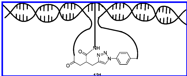
Figure 19. DNA templated CuAAC reaction product.
