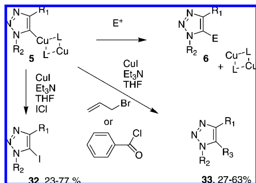
Scheme 4. Reaction of Electrophiles with Copper-Triazole Adduct 5
