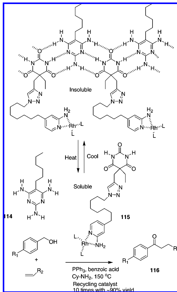
Figure 17. Catalysts and metal ligands derived through CuAAC.
