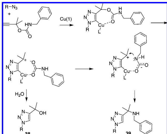
Scheme 6. Byproducts May Form from Alkynes Containing a Leaving Group in the \alpha -Position, Particularly if the Formed Carbenium Ion Is Stabilized a
