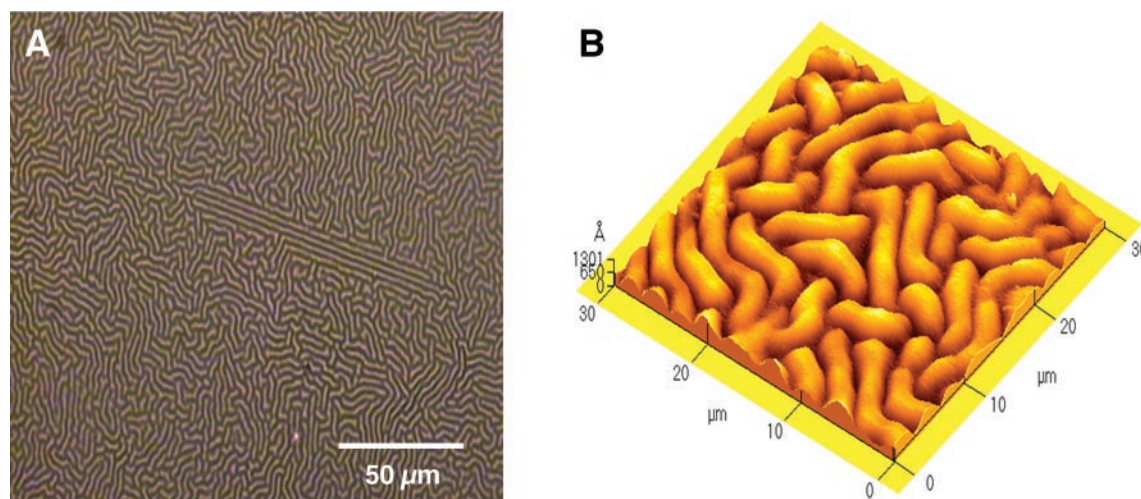
Fig. 1. (A) Reflection-mode optical micrograph of the lateral structure induced by an electric field applied across a polystyrene film capped by an Al layer acting as an electrode. The origin of the ordered region toward the center of the micrograph is currently under investigation. (B) AFM image taken using a tapping mode scan of the lateral morphology, showing the topography of the film surface. [Micrographs courtesy of S. Hutchinson and D. Bucknall]
