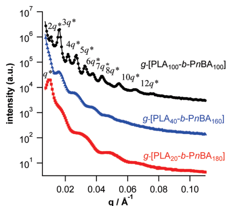
Figure 8. SAXS curves for brush block copolymers, g -[PLA- b -PnBA].
