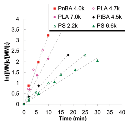
Figure 2. Dependence of \ln([\text{MM}]_0/[\text{MM}]_t) on time for ROMP of MMs. Conditions: [\text{MM}]_0 = 0.05 M in THF at room temperature, [\text{MM}/\text{C}]_0 = 200 . The dashed lines are best-fit lines.
