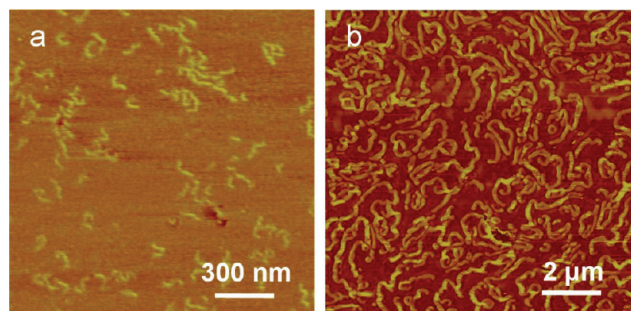
Figure 9. AFM phase images of (a) individual PLA brush homopolymers ( DP_{\text{backbone}} = 200 , MM NB(PLA)4.7k was used) on mica; (b) brush block copolymer, g -[PLA 100 - b -PnBA 100 ], morphology in thin film (ca. 120 nm) as cast from 2.5% toluene solution onto silicon wafer.
