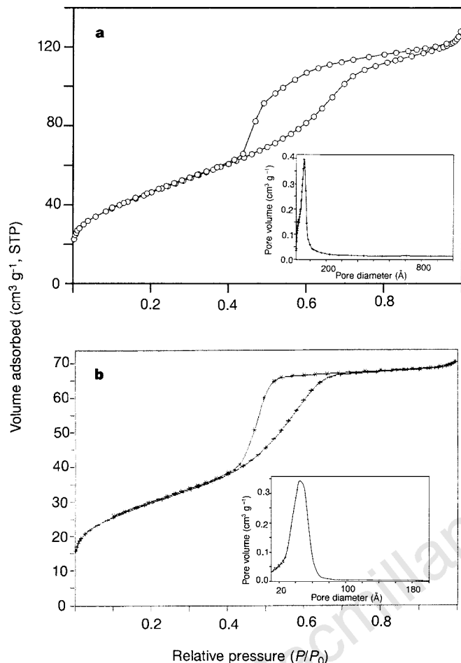
Figure 3 Nitrogen adsorption-desorption isotherms and pore-size distribution plots (insets) for calcined \text{TiO}_2 (a) and calcined \text{WO}_3 (b). Data were calculated using the BJH model from the adsorption branch isotherm. Both \text{TiO}_2 and \text{WO}_3 samples were calcined at 400^\circ\text{C} for 5 h in air. The isotherms were measured using a Micromeritics ASAP 2000 system. The samples were outgassed overnight at 200^\circ\text{C} before the analyses.
