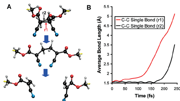
Figure 3. AI-SMD simulations of 1 using a force of 3 nN. (A) Snapshots along one trajectory for 1 showing selective cleavage ( t = 0, 200 , and 286 fs top to bottom). (B) Average bond lengths of 20 trajectories as a function of time for 1 , indicating sequential bond rupture of r1 and r2.
