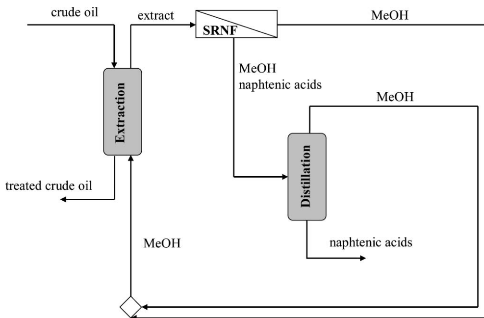
Fig. 15 Process scheme for crude oil deacidification (adapted from ref 297).
