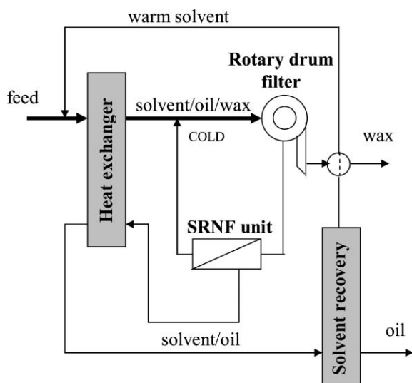
Fig. 13 Schematic representation of an SRNF-assisted lube oil dewaxing unit (adapted from ref. 287).
