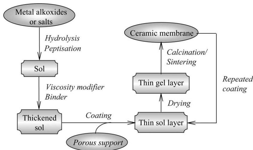
Fig. 8 Flow diagram for the preparation of microporous or mesoporous membranes via sol–gel techniques (taken from ref 31).
