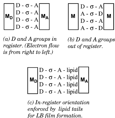
FIGURE 1. Alignment of D- \sigma -A molecules in monolayers.
