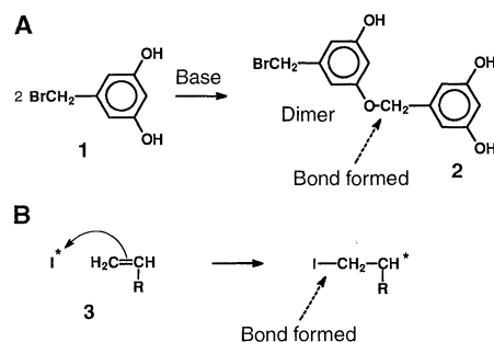
Scheme 1. (A) Typical polycondensation process. Addition does not create any new reactive centers. (B) Typical vinyl polymerization process. Addition creates a new reactive center.
