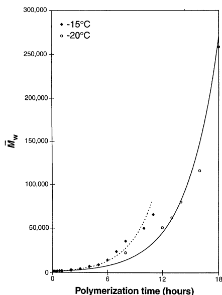
Fig. 1. Dependence of the weight-average molecular weight ( M_w ) of the polymers formed on the polymerization time.
