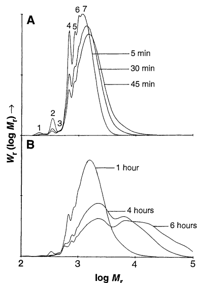
Fig. 2. Time dependence of the composition of the polymerization mixtures monitored by size exclusion chromatography [ M_r is plotted versus the mass-sensitive detector response W_r (\log M_r) in which W_r is the weight fraction at a particular M_r ]. (A) Initial stage. The numbers of the peaks represent the degree of polymerization for the corresponding oligomers. (B) Later stages.
