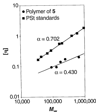
Fig. 3. Mark-Houwink-Sakurada plot for linear PST standards and poly-5 obtained in THF at 30°C.
