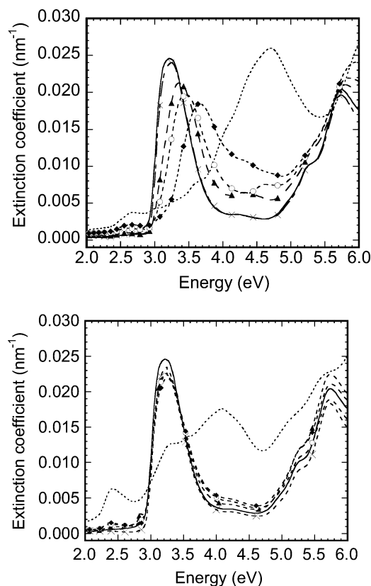
Figure 1. (a) The thin-film room temperature absorption spectra of compounds 10–15 . 10 [ \text{Ir}(\text{ppy}-\text{Br})_2(\text{acac}) ] dashed line with no markers, 11 [ \text{Ir}(\text{ppy}-\text{FH})_2(\text{acac}) ] has filled squares, 12 [ \text{Ir}(\text{ppy}-\text{FO}-\text{FH})_2(\text{acac}) ] has open circles, 13 [ \text{Ir}(\text{ppy}-(\text{FO})_2-\text{FH})_2(\text{acac}) ] has filled triangles, 14 [ \text{Ir}(\text{ppy}-(\text{FO})_{10})_2(\text{acac}) ] (same spectrum as 15 [ \text{Ir}(\text{ppy}-(\text{FO})_{30})_2(\text{acac}) ]) has crosses, and PFO has a solid line with no markers. (b) The thin-film room temperature absorption spectra of compounds 17–21 . 17 [ \text{Ir}(\text{btp}-\text{Br})_2(\text{acac}) ] dashed line with no markers, 18 [ \text{Ir}(\text{btp}-(\text{FO})_5)_2(\text{acac}) ] has filled squares, 19 [ \text{Ir}(\text{btp}-(\text{FO})_{10})_2(\text{acac}) ] has open circles, 20 [ \text{Ir}(\text{btp}-(\text{FO})_{20})_2(\text{acac}) ] has filled triangles, 21 [ \text{Ir}(\text{btp}-(\text{FO})_{40})_2(\text{acac}) ] has crosses, and PFO has a solid line with no markers.
