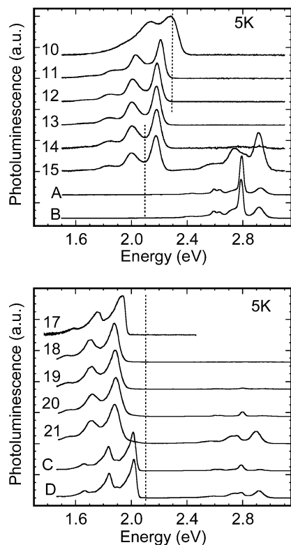
Figure 2. (a) The thin-film photoluminescence spectra at 5 K of compounds 10 [Ir(ppy-Br) 2 (acac)], 11 [Ir(ppy-(FH)) 2 (acac)], 12 [Ir(ppy-FO-FH) 2 (acac)], 13 [Ir(ppy-(FO) 2 -FH) 2 (acac)], 14 [Ir(ppy-(FO) 10 ) 2 (acac)], 15 [Ir(ppy-(FO) 30 ) 2 (acac)], blend A (same molecular percentage of [Ir(ppy) 2 (acac)] in PFO as for 14 ), and blend B (same molecular percentage of [Ir(ppy) 2 (acac)] in PFO as for 15 ). Spectra are normalized and offset along the vertical axis for ease of comparison. The dotted line indicates the position of the triplet state in PFO polymer at 2.1 eV and trimer at 2.3 eV. (b) The thin-film photoluminescence spectra at 5 K of compounds 17 [Ir(btp-Br) 2 (acac)], 18 [Ir(btp-(FO) 5 (acac)], 19 [Ir(btp-(FO) 10 ) 2 (acac)], 20 [Ir(btp-(FO) 20 ) 2 (acac)], 21 [Ir(btp-(FO) 40 ) 2 (acac)], blend C (same molecular percentage of [Ir(btp) 2 (acac)] in PFO as for 20 ), and blend D (same molecular percentage of [Ir(btp) 2 (acac)] in PFO as for 21 ). Spectra are normalized and offset along the vertical axis for ease of comparison. The dotted line indicates the position of the triplet state in PFO polymer at 2.1 eV.
