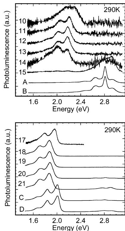
Figure 3. (a) The thin-film photoluminescence spectra at 290 K of compounds 10 [Ir(ppy-Br) 2 (acac)], 11 [Ir(ppy-FH) 2 (acac)], 12 [Ir(ppy-FO-FH) 2 (acac)], 13 [Ir(ppy-(FO) 2 -FH) 2 (acac)], 14 [Ir(ppy-(FO) 10 ) 2 (acac)], 15 [Ir(ppy-(FO) 30 ) 2 (acac)], blend A , and blend B . Spectra are normalized and offset along the vertical axis for ease of comparison. (b) The thin-film photoluminescence spectra at 290 K of compounds 17 [Ir(btp-Br) 2 (acac)], 18 [Ir(btp-(FO) 5 ) 2 (acac)], 19 [Ir(btp-(FO) 10 ) 2 (acac)], 20 [Ir(btp-(FO) 20 ) 2 (acac)], 21 [Ir(btp-(FO) 40 ) 2 (acac)], blend C , and blend D . Spectra are normalized and offset along the vertical axis for ease of comparison.
