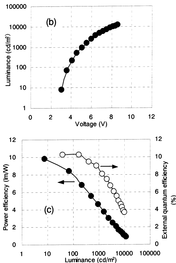
Figure 7. (a) OLED construction and molecular formulas of the compounds in each layer, (b) plot of luminance vs voltage, and (c) plots of power efficiency and external quantum efficiency vs luminance of the Ir(piq) 3 ( 7 ) device.
