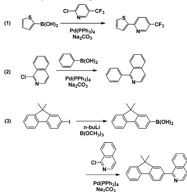
Scheme 1. Synthesis of the Ligands
