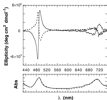
Fig. 1. CD and UV/vis spectra of two solutions ( 3\ \mu\text{M} ) of homoassociates of \text{H}_2\text{TPPS}_3^- corresponding to two characteristic experiments of Fig. 2B (vortex direction during the rotary evaporation; solid lines, CW; dashed lines, ACW). The bisignate CD signals are a consequence of the degenerate character of the transitions. The positive (negative) chirality sign is taken for CD bisignate signals at the absorption wavelength of the Soret(B)-band of the J-aggregate (490 nm) with positive (negative) values at high wavelengths. The CD samples consisted of relatively large volumes (1.5 ml to 3 ml), corresponding to representative volumes of the tested solutions (about 10 to 20% in volume in the case of the optimized experiments of Fig. 2).
