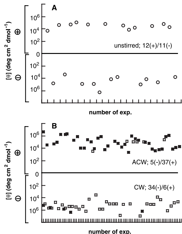
Fig. 2. (A) Chirality signs following from the pure symmetry breaking of unstirred solutions: 0.7 g of NaCl (0.6 M) was added to a 20 ml of a 3\ \mu\text{M} \text{Na}_3\text{TPPS}_3^- solution, previously sonicated for 30 min, and after its solubilization the aggregation process was started by the addition of 14\ \mu\text{l} of 98% \text{H}_2\text{SO}_4 . (B) Chirality signs following the biased symmetry breaking caused by vortex motion: concentration of 500 ml of 0.12\ \mu\text{M} solutions of \text{H}_2\text{TPPS}_3^- (prepared from the trisodium salt, with the addition of 14\ \mu\text{l} of \text{H}_2\text{SO}_4 and 0.5 g of NaCl) was conducted by rotary evaporation ( 600 \pm 50 rpm, inclination of 45^\circ , 55^\circ\text{C} , and 25 torr) (blank squares, CW; solid squares, ACW) to 20 ml (i.e., to the same concentrations as for the experiments of Fig. 1); rotary evaporation typically takes about 2 hours. In the case of unstirred solutions (A), the ellipticity values increase with time up to a constant, and CD spectra were typically recorded after 3 hours of aggregation. For stirred solutions (B), the CD spectra were recorded immediately after finishing the experiment, but no substantial changes in ellipticity values were detected after several months.
