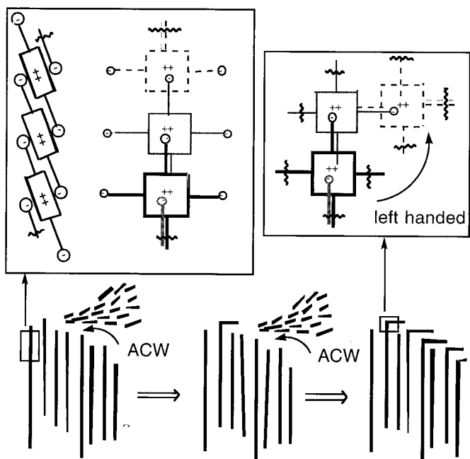
Fig. 3. Two-dimensional schematic picture of the autocatalytic process leading to chiral selection in the supramolecular association of the substituted porphyrins. Diastereotropic relative motion of oligomeric blocks and steric hindrance effects on the folding of the J-chains by aggregation would explain sign induction by vortical stirring. Insets show the three-dimensional extended chromophores in J-aggregates of diprotated porphyrins. According to the exciton coupling model for \pi systems (22) a right-handed (left-handed; i.e., the case shown in the inset of Fig. 3) chirality results in a +(-) chirality sign. Then ACW (CW) vortex would generate a left-handed (right-handed) chirality.
