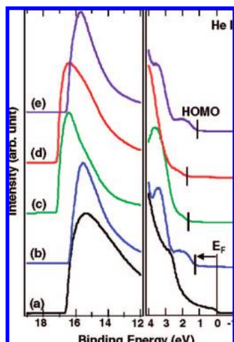
Figure 1. UPS spectra of (a) Au reference, (b) PFN-Br , (c) PFN + Br - , (d) PFN + BIIm 4 - , and (e) PFNSO 3 - Na + . LHS: High binding energy cutoff region. The intensity is normalized relative to the maximum point. RHS: HOMO region. The intensities are magnified along the ordinate to highlight spectral comparison.
