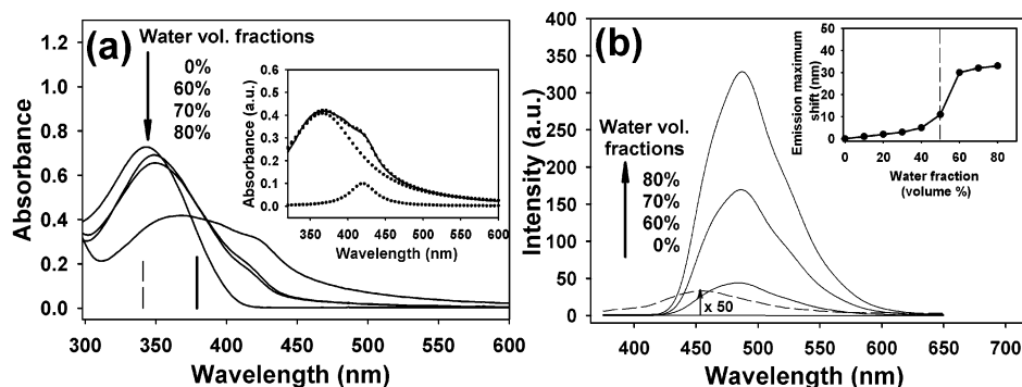
Figure 3. (a) UV absorption spectra changes of CN-MBE ( 2 \times 10^{-5} \text{ mol L}^{-1} ) depending on the water fractions in THF. The calculated absorption maximum peaks of twisted (dot line) and planar form (solid line) of CN-MBE are shown at the bottom. Inset shows peak separation of CN-MBE nanoparticles in the case of 80% water addition. (b) PL spectra changes of CN-MBE ( 2 \times 10^{-5} \text{ mol L}^{-1} ) depending on the water fractions in THF. Inset shows the change in the emission maximum peak of CN-MBE.
