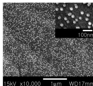
Figure 1. SEM images of CN-MBE nanoparticles obtained from nanoparticles' suspension containing 80% volume fractions of water in THF. Inset shows the magnified SEM image.
