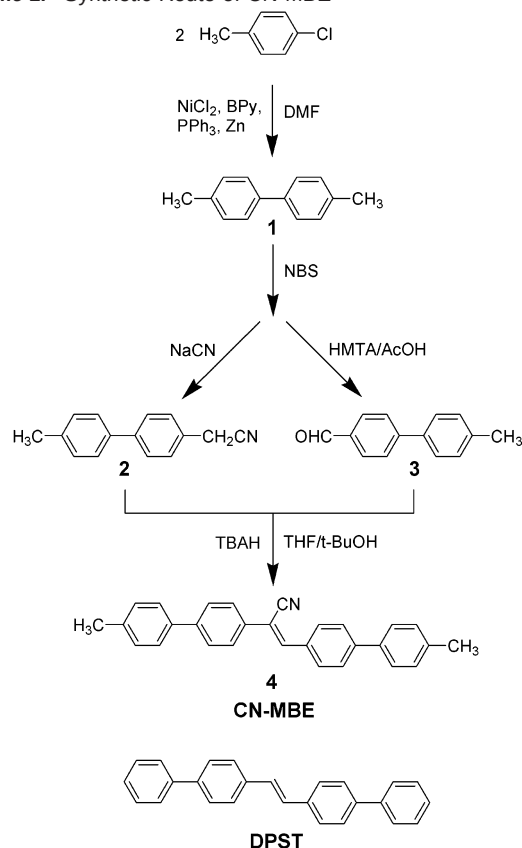
Scheme 2. Synthetic Route of CN-MBE
