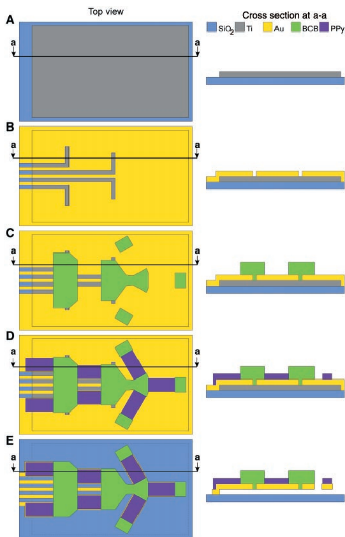
Fig. 1. A schematic drawing of the process steps for fabricating the microrobotic arms (in this case, an arm with three fingers). (A) Deposition and patterning of the sacrificial Ti layer. (B) Deposition of the structural Au layer and etching of the isolating slits. (C) Patterning of the BCB rigid elements. (D) Electrodeposition of PPy. (E) Etching of the final robot and electrode structure, removal of the sacrificial layer. Each micro-actuator is 100 \mu\text{m} by 50 \mu\text{m} . The total length of the robot is 670 \mu\text{m} , and the width at the base is either 170 or 240 \mu\text{m} (depending on the wire width, which was either 10 or 20 \mu\text{m} , respectively).
