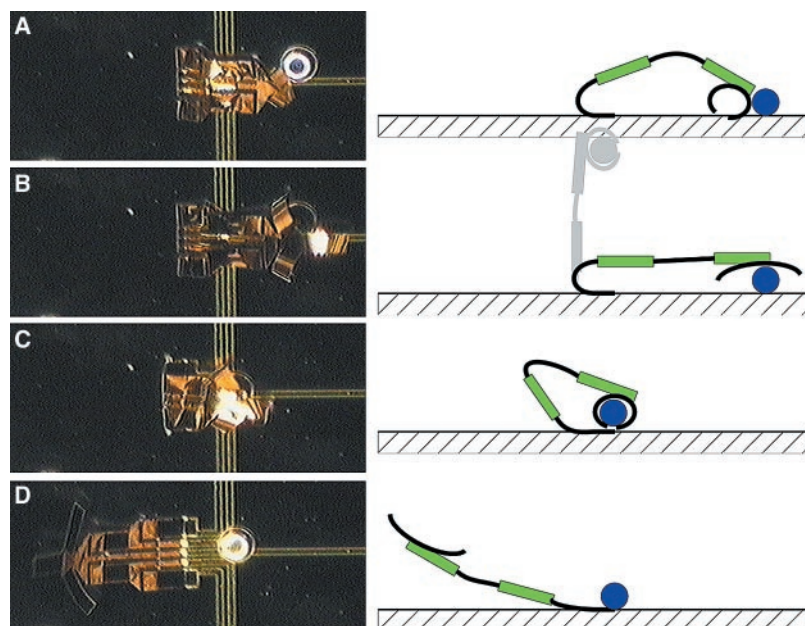
Fig. 2. (A through D) A sequence of pictures (left) showing the grabbing and lifting of a 100\text{-}\mu\text{m} glass bead and schematic drawings of the motion (right). In this case, the arm has three fingers, placed at 120^\circ from each other. The pictures do not illustrate the fact that the bead is actually lifted from the surface before it is placed at the base of the robot arm. We have illustrated this in gray in the second sketch to the right. A film showing the full movement can be seen online (16).
