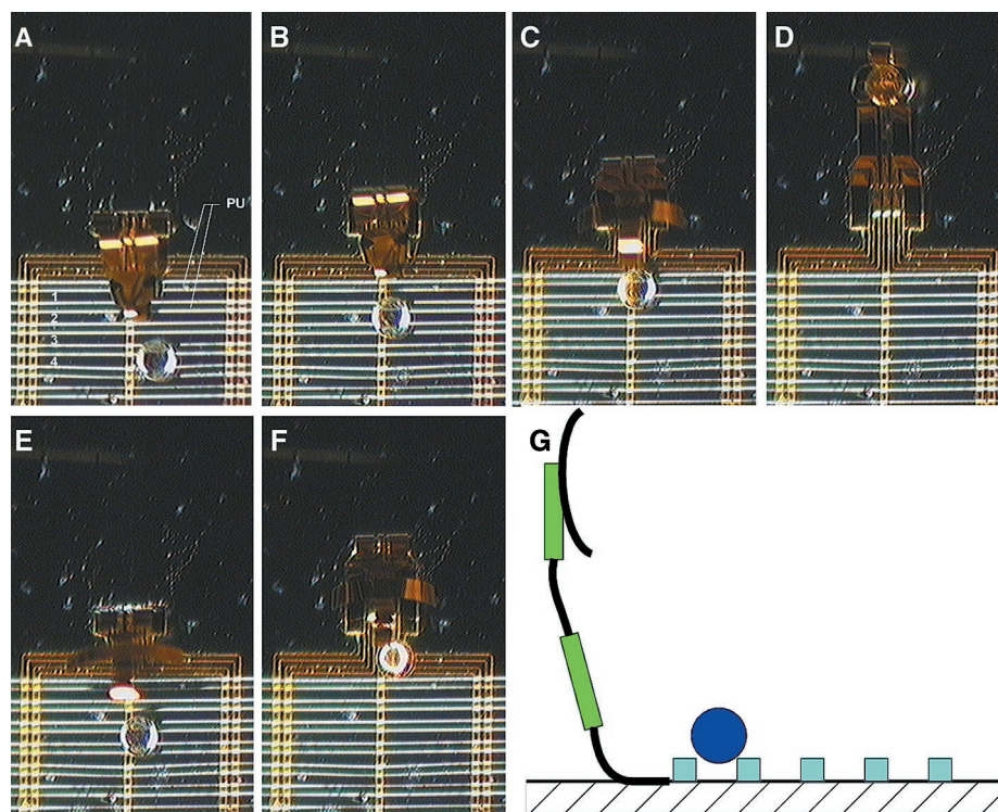
Fig. 3. (A through F) Picture sequence of moving a 100\text{-}\mu\text{m} glass bead over a polyurethane track system (16). The distance between two tracks is 60\text{ }\mu\text{m} . We picked up the glass bead and moved it from track 4 to 2, to 1, and to 3, and finally to the base of the robot outside of the tracks. The total maximum displacement of the glass bead was \sim 270\text{ }\mu\text{m} . In this case, the robot had three fingers placed at 90^\circ from each other. In (D), the robot arm is fully retracted with the glass bead held in its fingers. (G) Schematic of the experimental layout.
