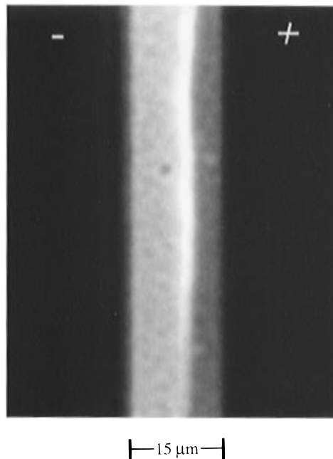
Figure 7. An optical microphotograph of the Au/PPV + PEO/Au LEC (surface cell configuration) during operation. A 4 V bias is being applied between the pair of gold electrodes which are separated by 15 μm. Green light is emitted from the narrow p-n junction near the center of the spacing. This figure, presented here in black and white, is available in color on the World Wide Web. See Supporting Information paragraph on any current masthead page for instructions on accessing the images.
