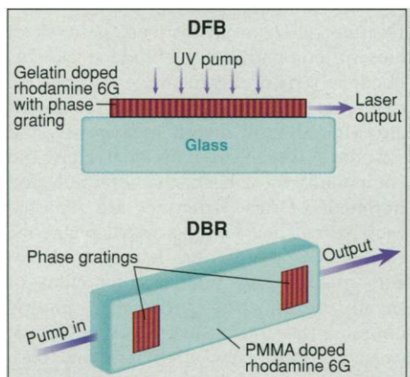
Schematic structures of the first DFB (top) and DBR (bottom) lasers. In the DFB laser, feedback is provided throughout the gain region by a phase grating that was defined in the gelatin by intersecting ultraviolet beams. In the DBR laser, the gratings are defined at the ends of the laser cavity. [Adapted from (3, 4)]
