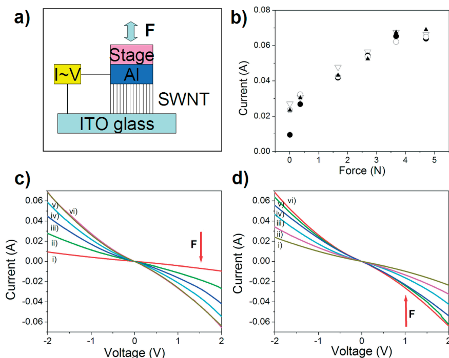
Figure 4. a) A schematic setup for the I - V measurements – Note, the drawing is not to scale; b) Current ( I ) vs. the applied force for a VA-SWNT film on an ITO glass at 2 V (solid circles: 1st pressing cycle, open circles: 1st depressing cycle; solid triangles: 2nd pressing cycle, open triangles: 2nd depressing cycle); c) I - V curves of a VA-SWNT film on ITO glass during the 1st pressing cycle (i, 0.01; ii, 0.36; iii, 1.67; iv, 2.70; v, 3.68; vi, 4.70 N); d) I - V curves of a VA-SWNT film on ITO glass during the 1st depressing cycle (vi, 4.70; v, 3.68; iv, 2.70; iii, 1.67; ii, 0.36; i, 0.01 N). Samples size: (ca. 3 mm \times 3 mm).
