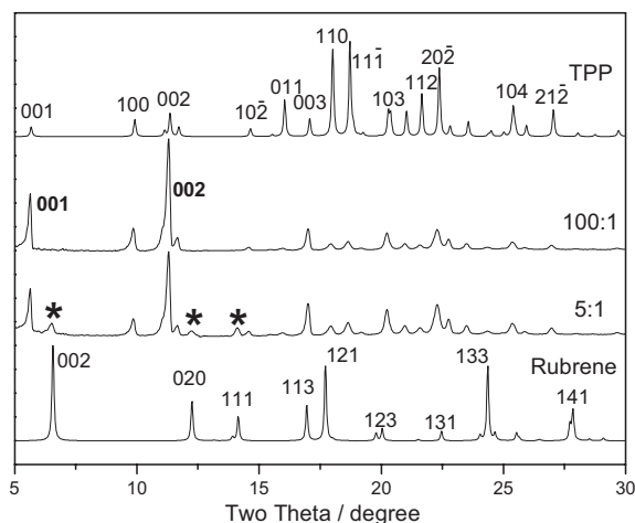
Figure 3. XRD patterns of the 1D nanomaterials with TPP/rubrene molar ratios of 100:1 and 5:1. The stars indicate the diffraction peaks of rubrene. For comparison, the patterns of TPP and rubrene powders are also displayed.
