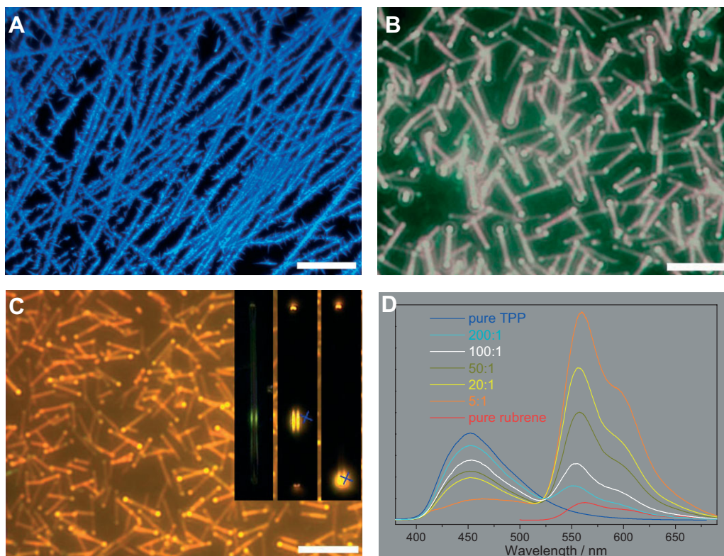
Figure 4. A–C) Fluorescence microscopy images of the nanostructures with different rubrene contents. A) Pure TPP, excited with UV (330–385 nm), B) 100:1 or molar TPP/rubrene, excited with UV, C) pure rubrene, excited with blue light (460–490 nm); all scale bars are 5 \mu\text{m} . D) Emission spectra of the nanowires deposited onto quartz wafers with different rubrene contents. Insets: Bright-field image (left), and micro-area fluorescence images of a single nanorod obtained by exciting the middle part (middle) and top area (right) using a focused laser. The blue crosses indicate the excitation position.
