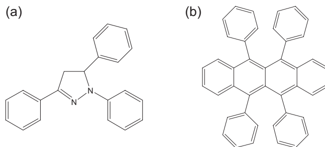
Scheme 1. Molecular structures of TPP (A) and rubrene (B).
