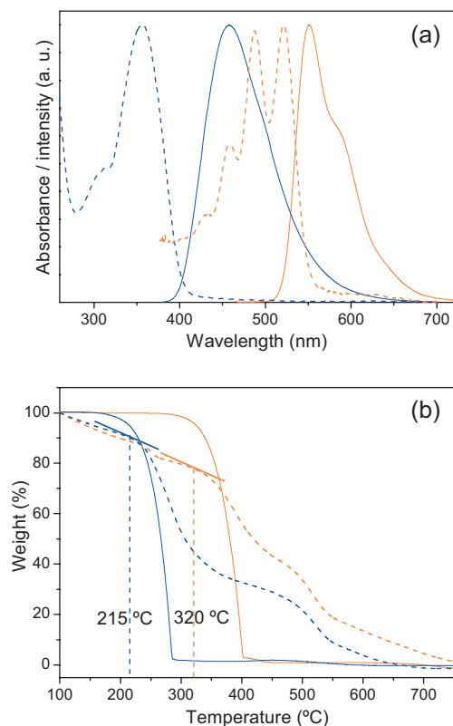
Figure 1. A) Absorption (dashed) and fluorescence emission (solid) spectra of TPP (blue) and rubrene (orange) monomers in ethanol. B) TGA plots of pure dyes (solid) and the mixtures of adsorbent and dye with w/w ratio of 100:1 (dashed). All plots were measured in nitrogen atmosphere at a heating rate of 10^{\circ}\text{C min}^{-1} , and the weights of dyes were normalized to 100 %.
