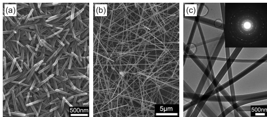
Figure 2. FE-SEM (A,B) and TEM (C) images of the binary nanostructures with a TPP/rubrene molar ratio of 100:1 prepared under different conditions. Inset: SAED pattern of the nanowires.
