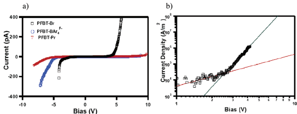
Figure 6. (a) Average I - V curves for PFBT-Br (black), PFBT-BAr 4 F- (blue), and PFBT-Pr (red) and (b) the current density versus bias for PFBT-Br . Solid lines are fits to the SCLC with shallow traps model (see Experimental Section).
