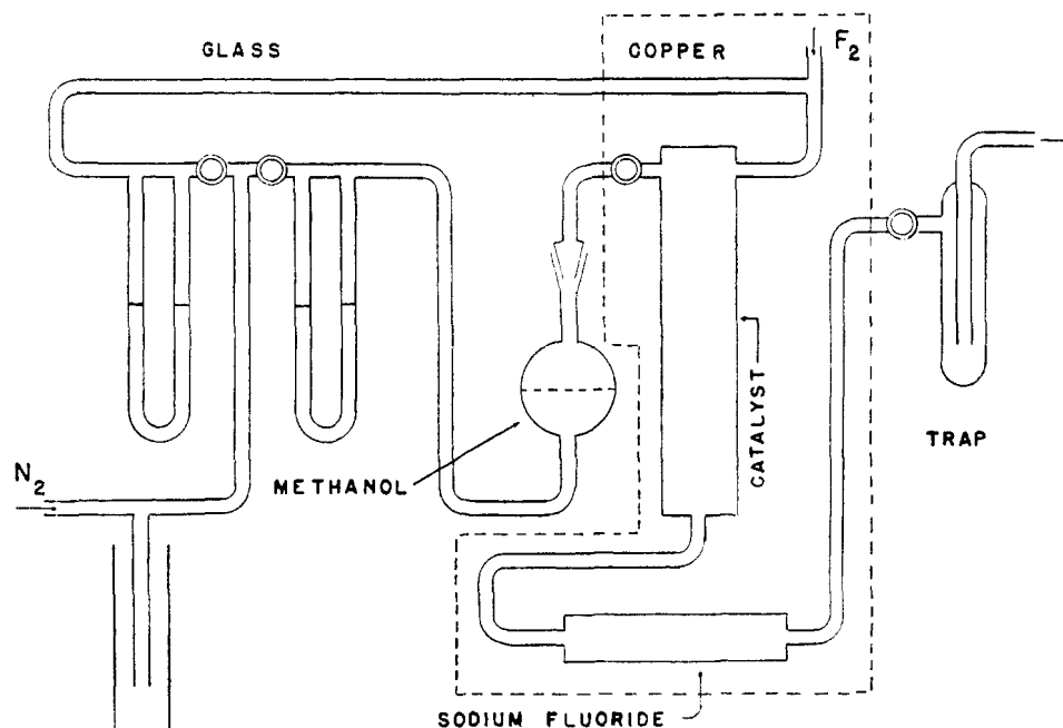
Fig. 1.—Catalytic system.
