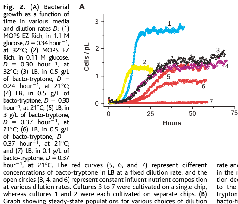
Fig. 2. (A) Bacterial growth as a function of time in various media and dilution rates D : (1) MOPS EZ Rich, in 1.1 M glucose, D = 0.34 \text{ hour}^{-1} , at 32^\circ\text{C} ; (2) MOPS EZ Rich, in 0.11 M glucose, D = 0.30 \text{ hour}^{-1} , at 32^\circ\text{C} ; (3) LB, in 0.5 g/L of bacto-tryptone, D = 0.24 \text{ hour}^{-1} , at 21^\circ\text{C} ; (4) LB, in 0.5 g/L of bacto-tryptone, D = 0.30 \text{ hour}^{-1} , at 21^\circ\text{C} ; (5) LB, in 3 g/L of bacto-tryptone, D = 0.37 \text{ hour}^{-1} , at 21^\circ\text{C} ; (6) LB, in 0.5 g/L of bacto-tryptone, D = 0.37 \text{ hour}^{-1} , at 21^\circ\text{C} ; and (7) LB, in 0.1 g/L of bacto-tryptone, D = 0.37 \text{ hour}^{-1} , at 21^\circ\text{C} . The red curves (5, 6, and 7) represent different concentrations of bacto-tryptone in LB at a fixed dilution rate, and the open circles (3, 4, and 6) represent constant influent nutrient composition at various dilution rates. Cultures 3 to 7 were cultivated on a single chip, whereas cultures 1 and 2 were each cultivated on separate chips. (B) Graph showing steady-state populations for various choices of dilution
