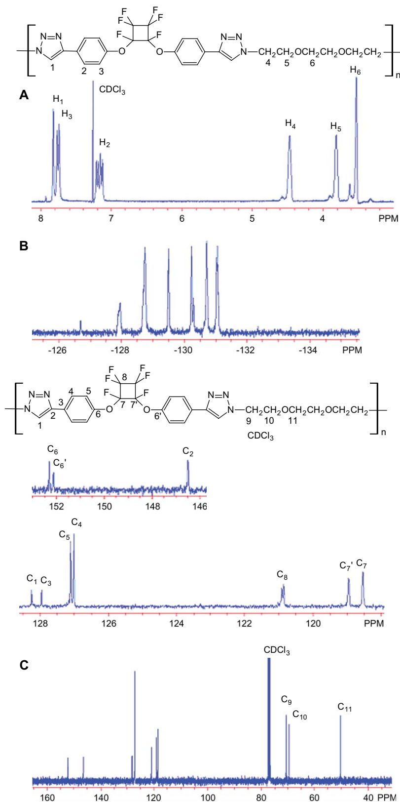
Fig. 4. ^1\text{H} NMR (A), ^{19}\text{F} NMR (B) and ^{13}\text{C} NMR (C) spectra of polymer 7a .
