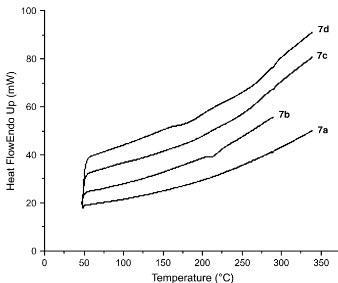
Fig. 6. DSC analysis of polymer 7a–d at 20\text{ }^\circ\text{C}/\text{min} .
