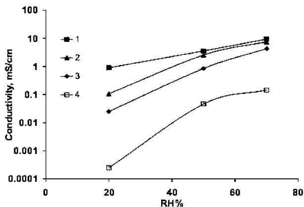
Figure 14. Conductivity of new composite materials compared with Nafion at 120 °C and different relative humidity (RH): (1) Nafion115; (2) 40% poly(VDF-co-CTFE) copolymer/60% sulfonated silicon dioxide; (3) poly(VDF-co-CTFE)-g-SPETMS; (4) 30% poly(VDF-co-CTFE)/30% Nafion/40% MS). Reproduced with permission from ref 139. Copyright 2007 Electrochemical Society.
